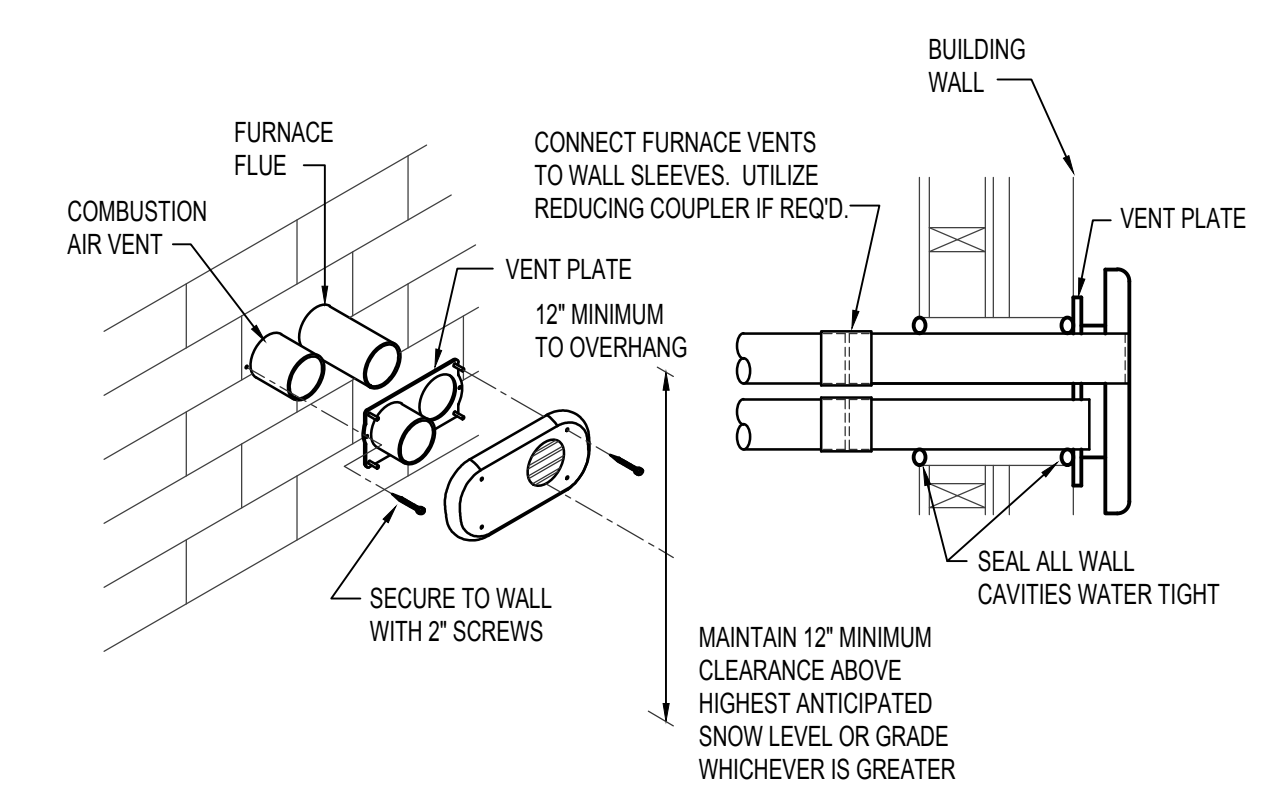
FURNACE VENT TERMINATION DETAIL NO SCALE
