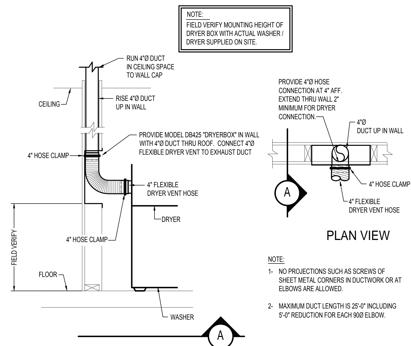
DRYER VENT DETAIL NO SCALE
