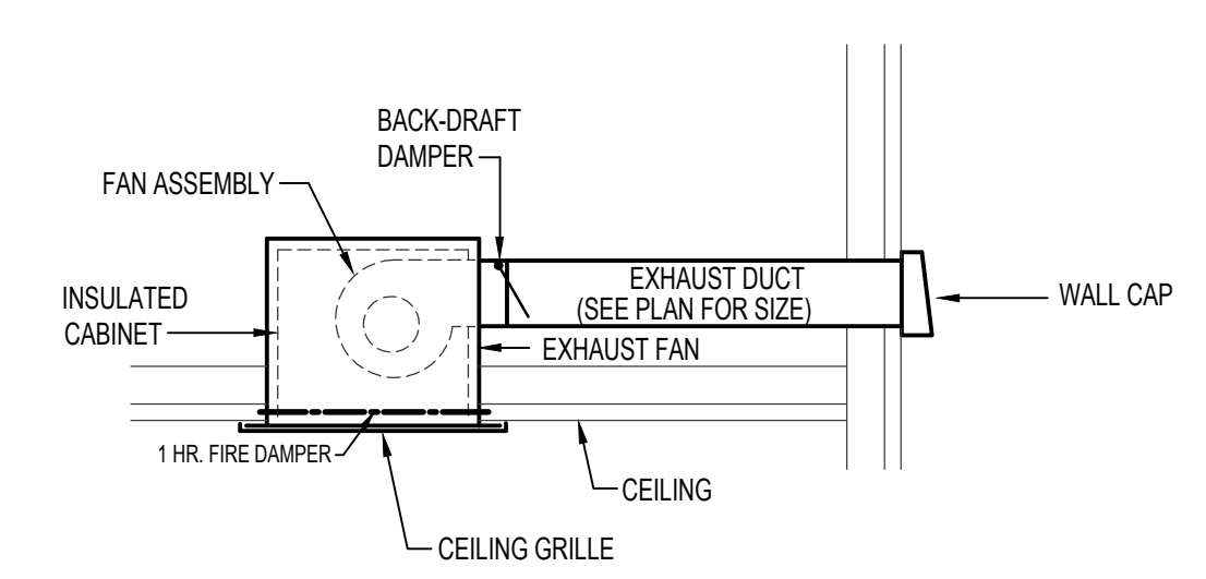
CEILING MOUNTED EXHAUST FAN DETAIL NO SCALE
